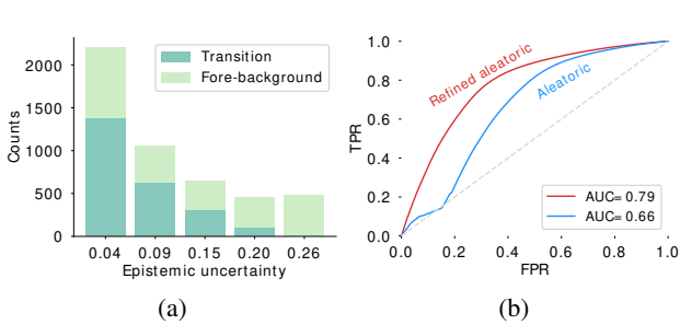
Figure 6. The correlation regions of decomposed uncertainties. The proportion of foreground and background regions is higher in high epistemic uncertainty. ROC of the obtained regions and the real transition regions, refined aleatoric uncertainty-based algorithm achieves better performance.
