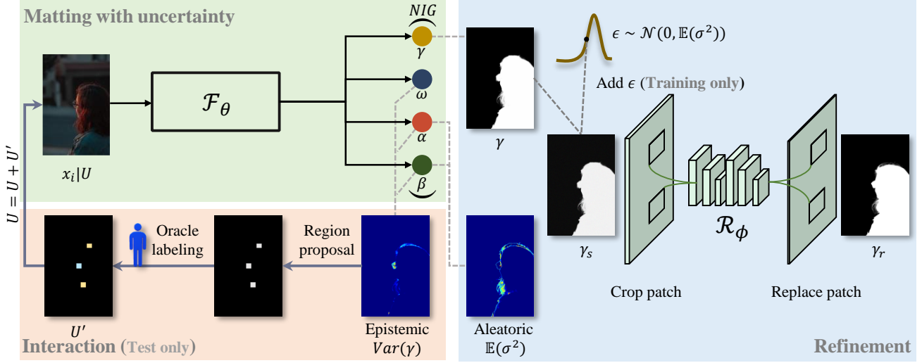
Figure 2. Illustration of the proposed decomposed-uncertainty-guided matting framework. The matting network fits a NIG distribution, proposing interactive regions for user based on epistemic uncertainty and detail regions for refined module based on aleatoric uncertainty.
