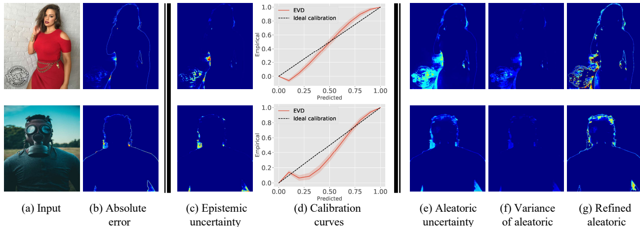
Figure 8. Uncertainty evaluation of MODNet. Epistemic uncertainty matches error regions in most time. Aleatoric uncertainty may capture erroneous transition regions, the variance of aleatoric uncertainty can help to more precisely indicate transition regions.
