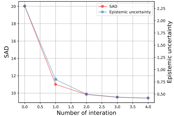
Figure 7. SAD and epistemic uncertainty at different number of interaction.
